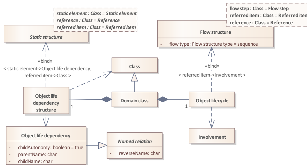
Figure 22: Domain class definition
